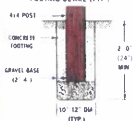
FOOTING DETAIL (TYP)
